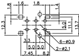
P.C.B MOUNTING HOLES
