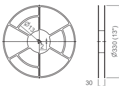
13" Reel
